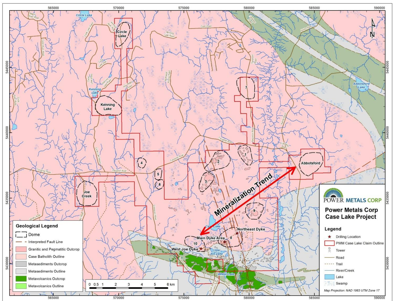
Figure 1. Case Lake property with Spodumene bearing LCT pegmatites on a 10 km mineralization trend.
